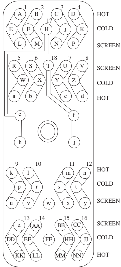
VIEW ON WIRING SIDE
