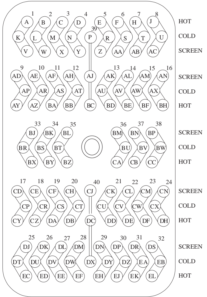
VIEW ON WIRING SIDE
